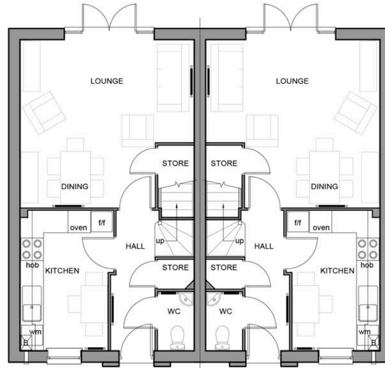
GROUND FLOOR PLAN Barwick Barwick
