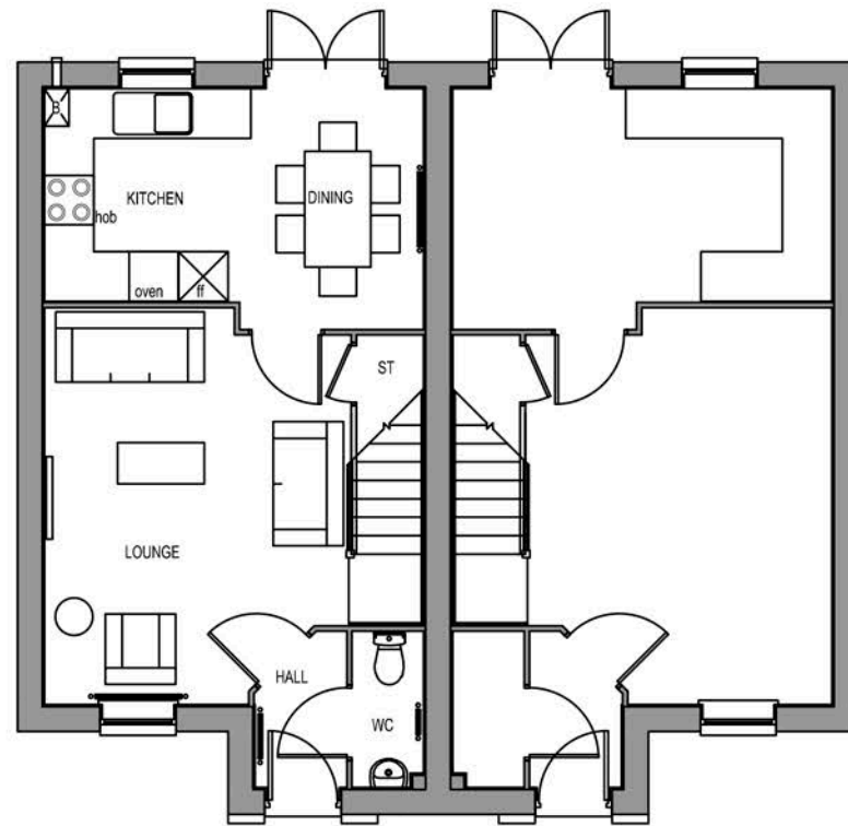
GROUND FLOOR PLAN Dewsbury Dewsbury
