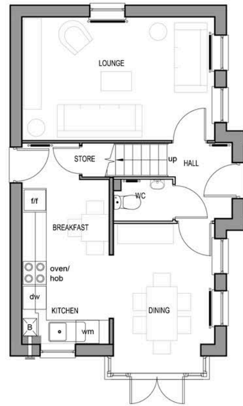
GROUND FLOOR PLAN Morpeth
