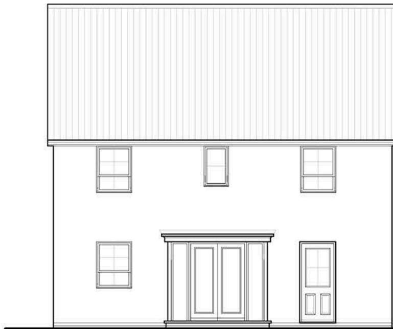
REAR ELEVATION Somerton
