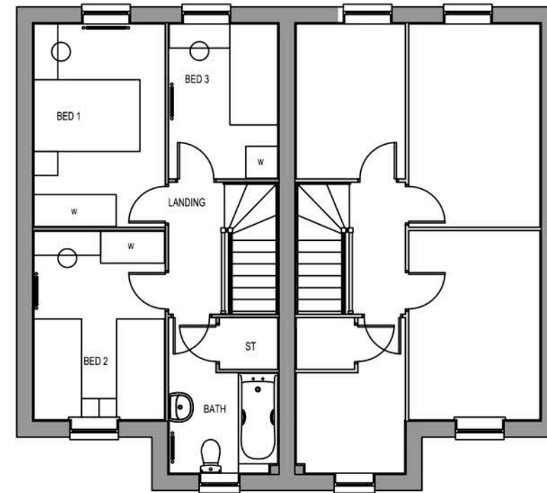
FIRST FLOOR PLAN Dewsbury Dewsbury
